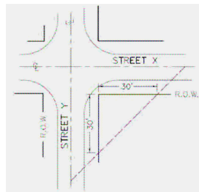
Illustration 6-2. Sight distance triangle.
