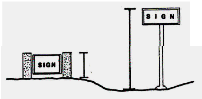
Illustration 6-7: Sign height computation in cases where the normal grade cannot reasonably be determined
