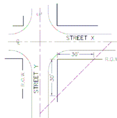
Illustration 6-1. Visual clearance.
